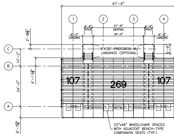
SEATING PLAN SCALE: 3/32" = 1'-0"
