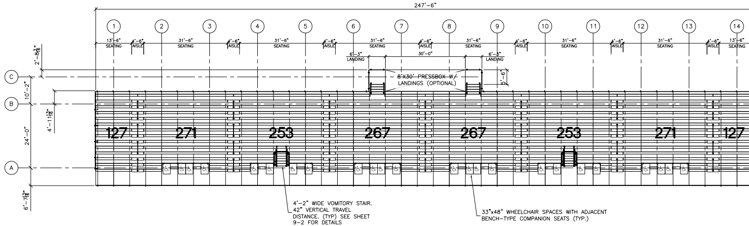
SEATING PLAN SCALE: 3/32" = 1'-0"
