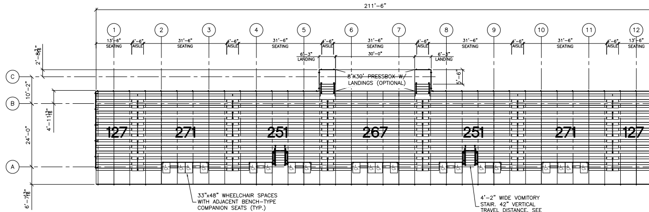
SEATING PLAN SCALE: 3/32" = 1'-0"
