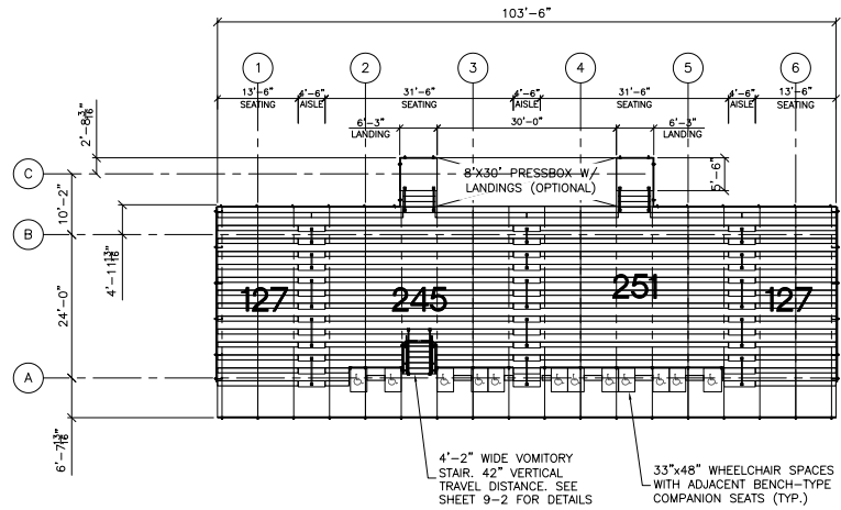
SEATING PLAN SCALE: 3/32" = 1'-0"
