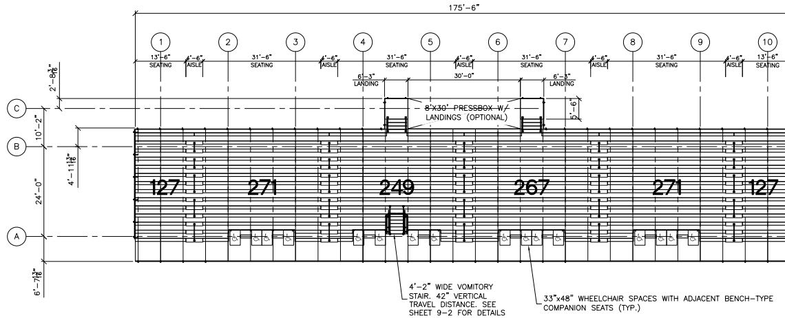
SEATING PLAN SCALE: 3/32" = 1'-0"
